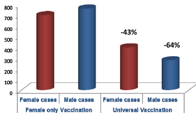
Fig. 2. Reduction of the remaining HPV-16,-18-anal cancer burden in females and males in Europe through female-only HPV vaccination and universal HPV vaccination (age 12 years, 70% VCR).
